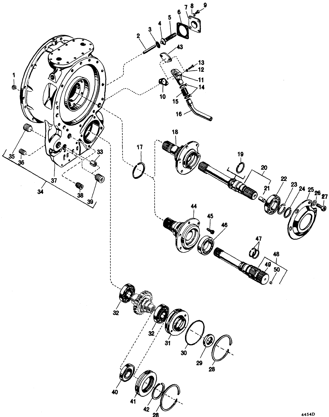
FIG 4. TORQUE CONVERTER HOUSING
