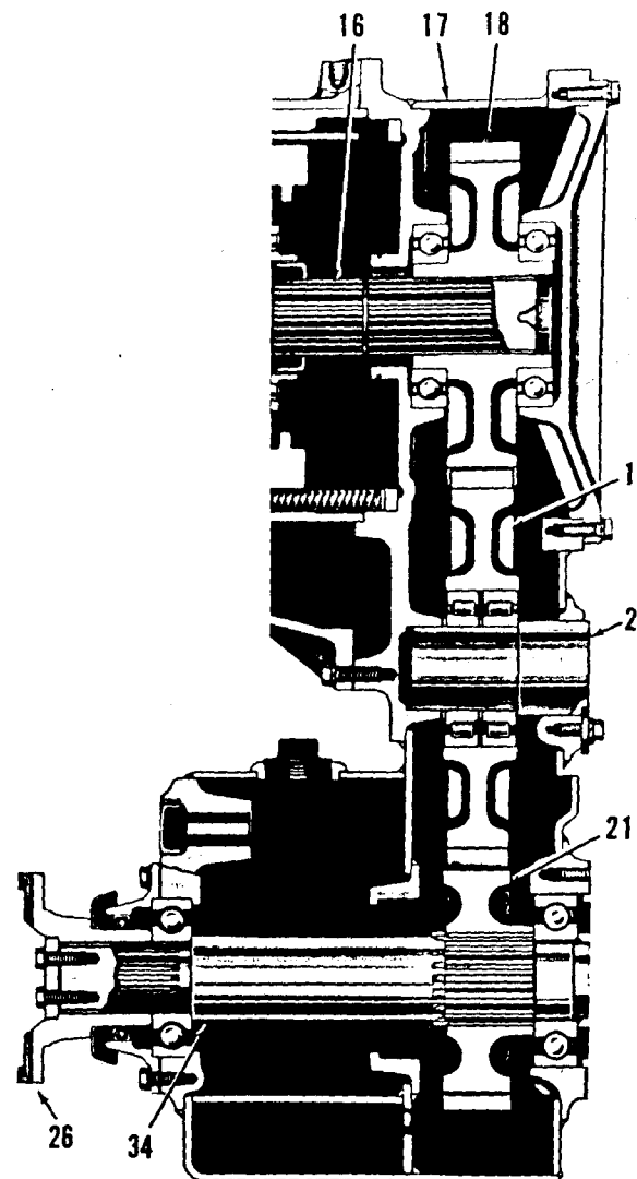
CRT 3321-1 TRANSMISSION TRANSFER GEARS WITHOUT DISCONNECT
