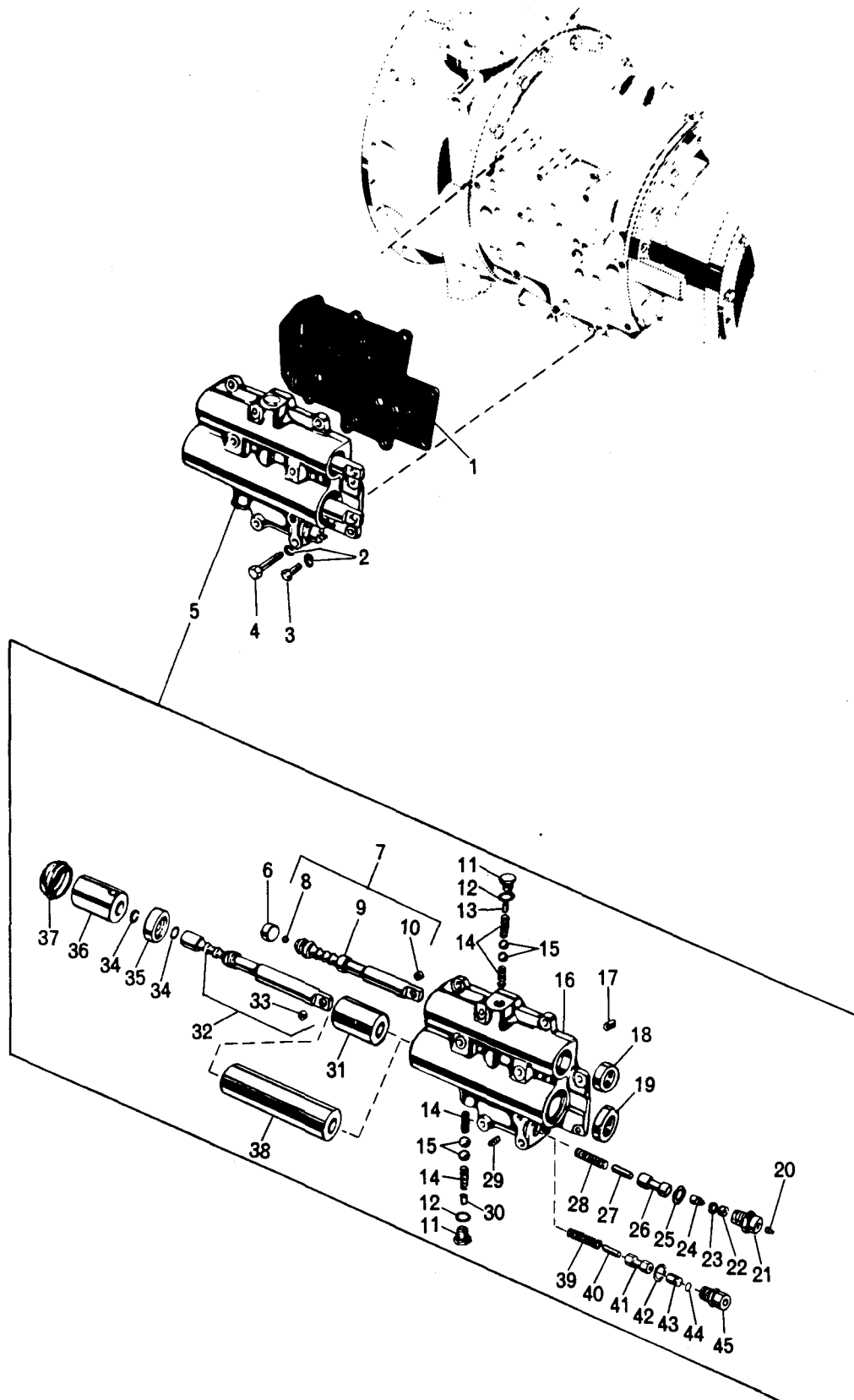
FIG 13-1. CONTROL VALVE BODY
