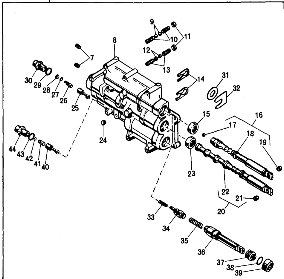
FIG 13. CONTROL VALVE BODY
