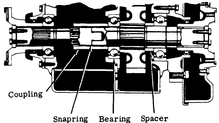
Fig. 2. Standard configuration
