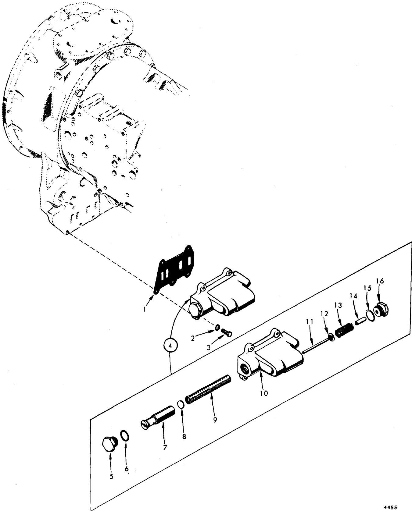
FIG 14. MAIN PRESSURE REGULATOR VALVE
