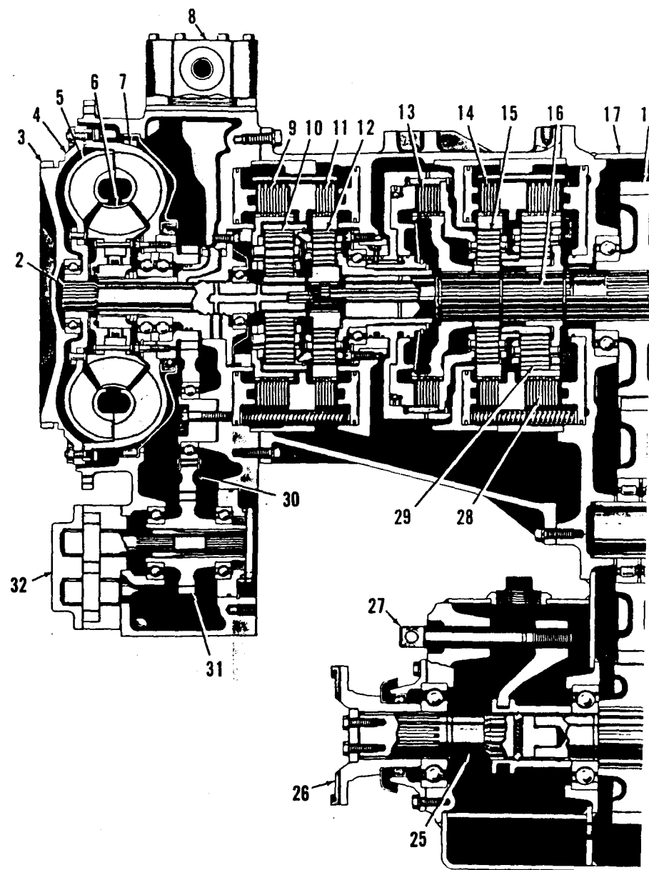
CRT 3331-1 TRANSMISSION - WITH FRONT DISCONNECT (ENGINE MOUNTED-GEAR DRIVEN)
