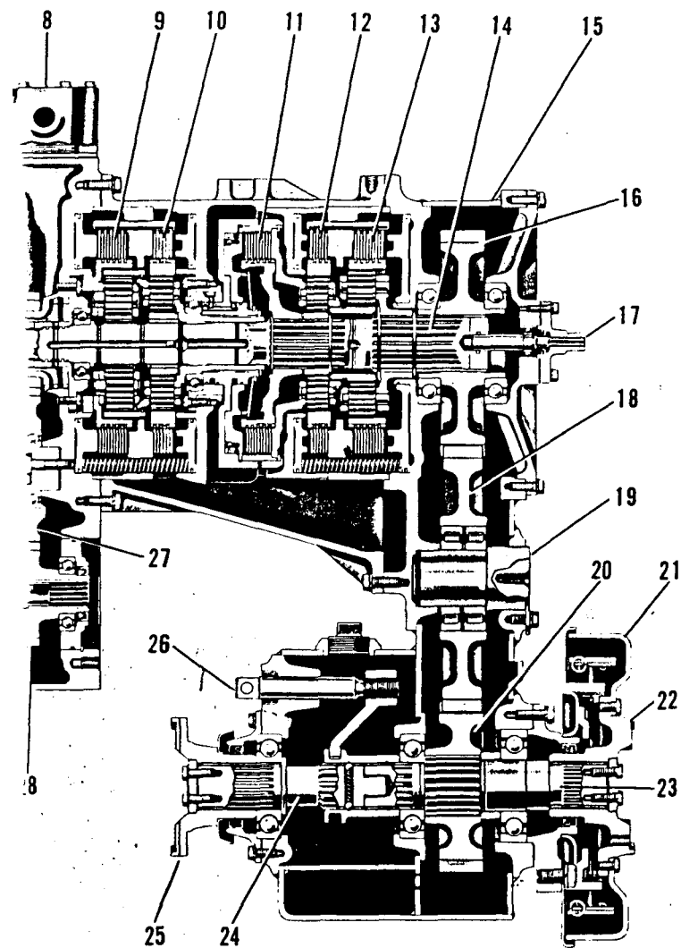
TRANSMISSION ENGINE MOUNTED AR DRIVE AND FRONT OUTPUT DISCONNECT
