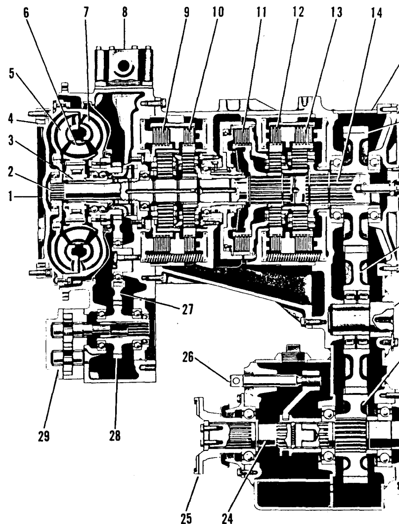
TRANSMISSION ENGINE MOUNTED (GEAR DRIVE AND FRONT OUTPUT DISCONNECT)
