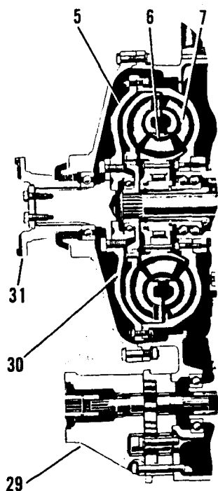
REMOTE MOUNTED (FLANGE DRIVE)
