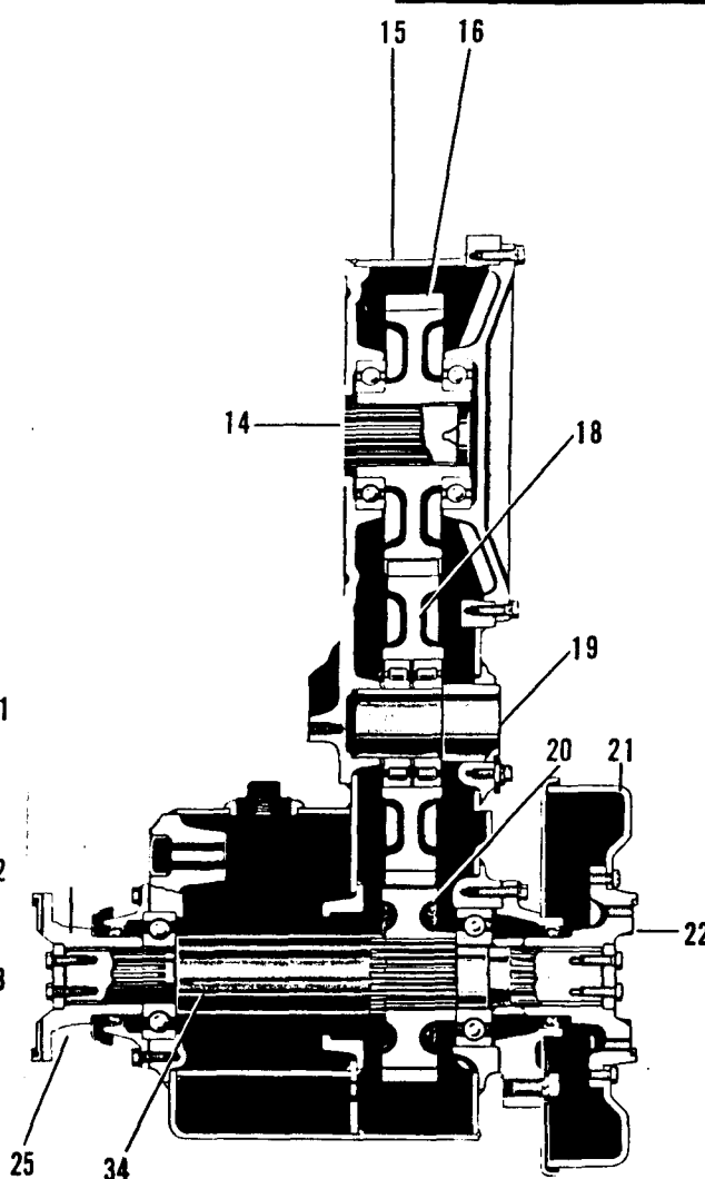
TRANSFER GEAR SECTION (WITHOUT DISCONNECT)
