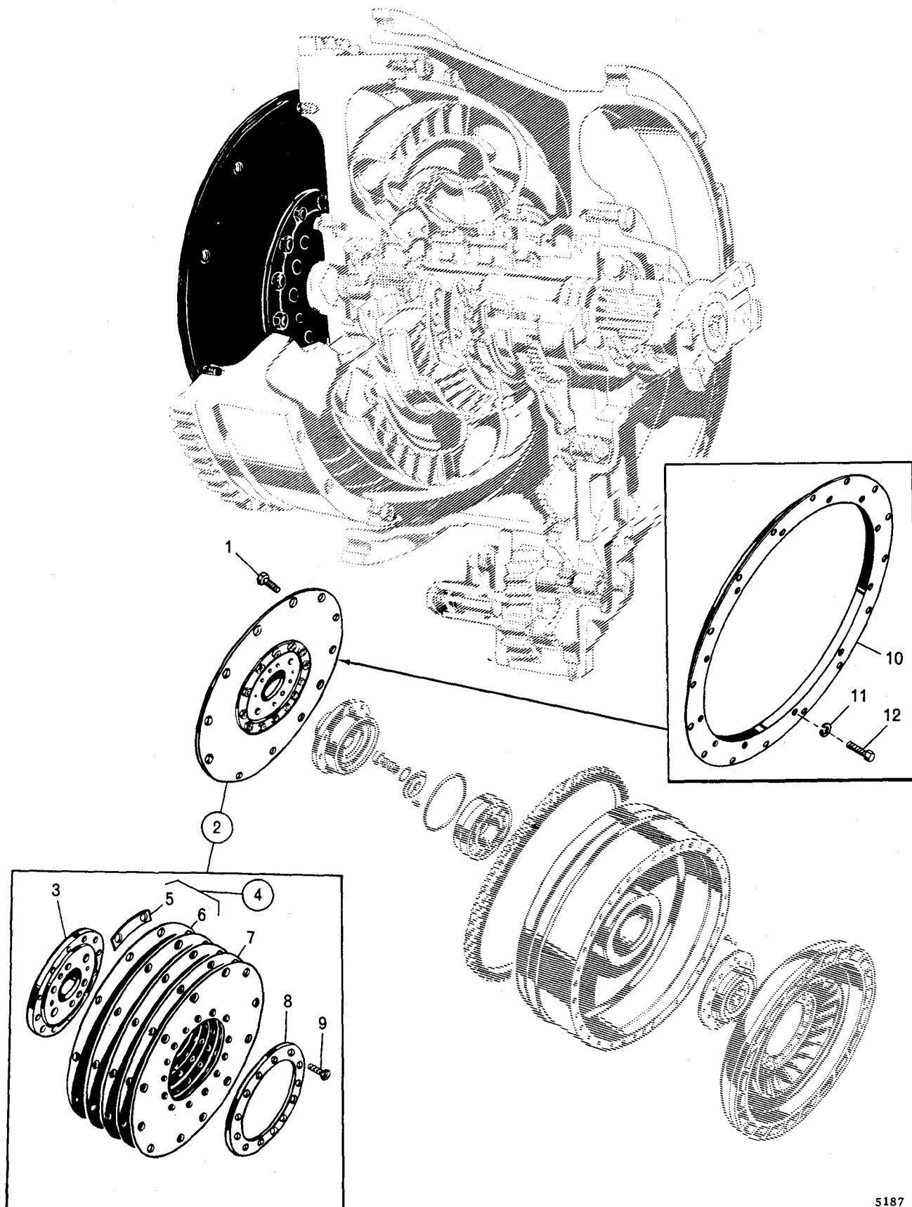
FIG. 7. FLEXIBLE FLYWHEEL DISK
