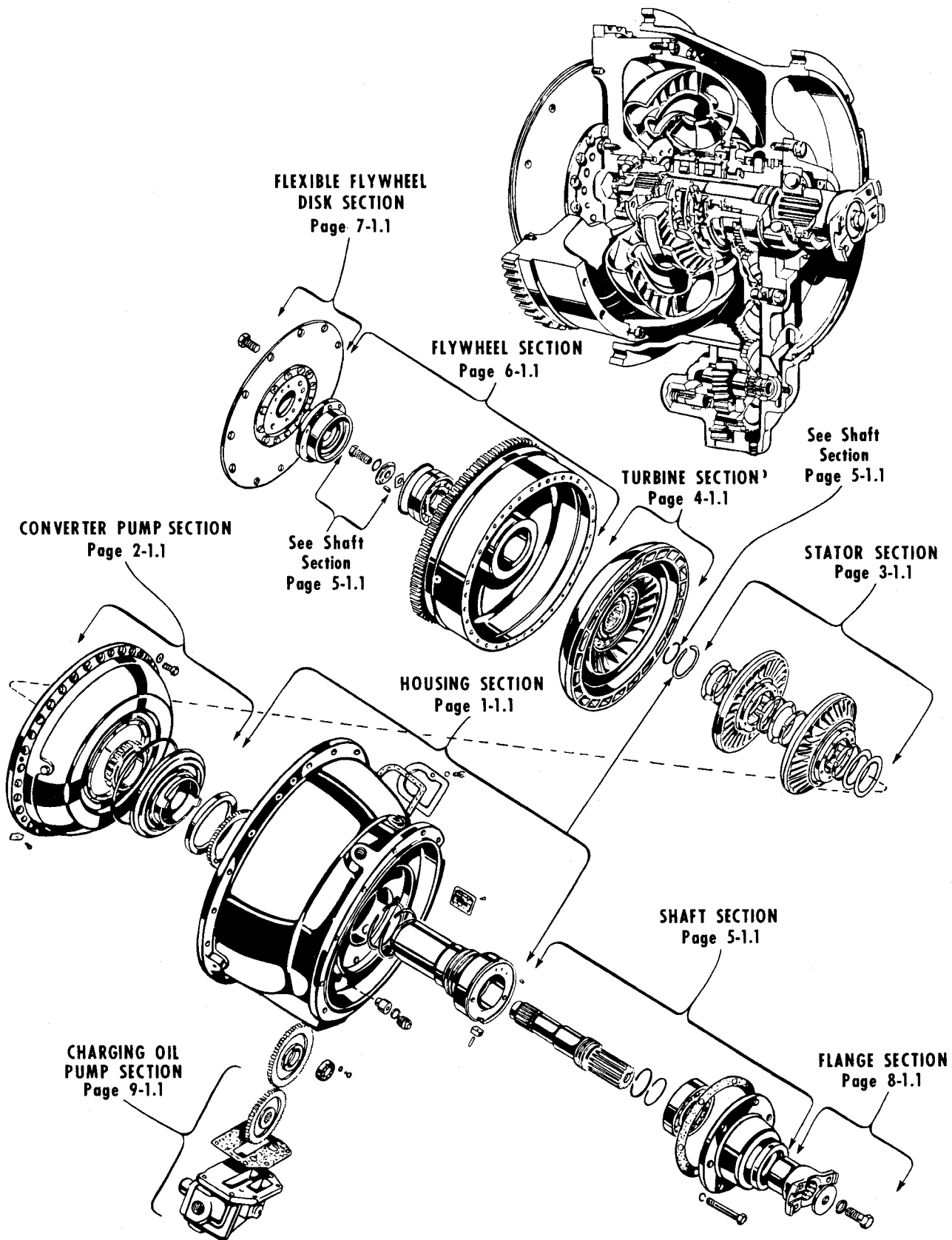
PICTORIAL INDEX, BASIC CONVERTER
