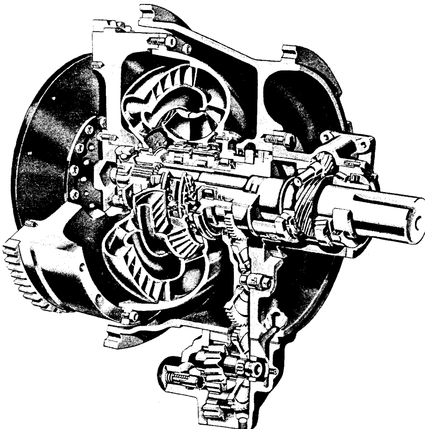
FIG. 10. ALLISON MODEL TCA TORQMATIC CONVERTER
