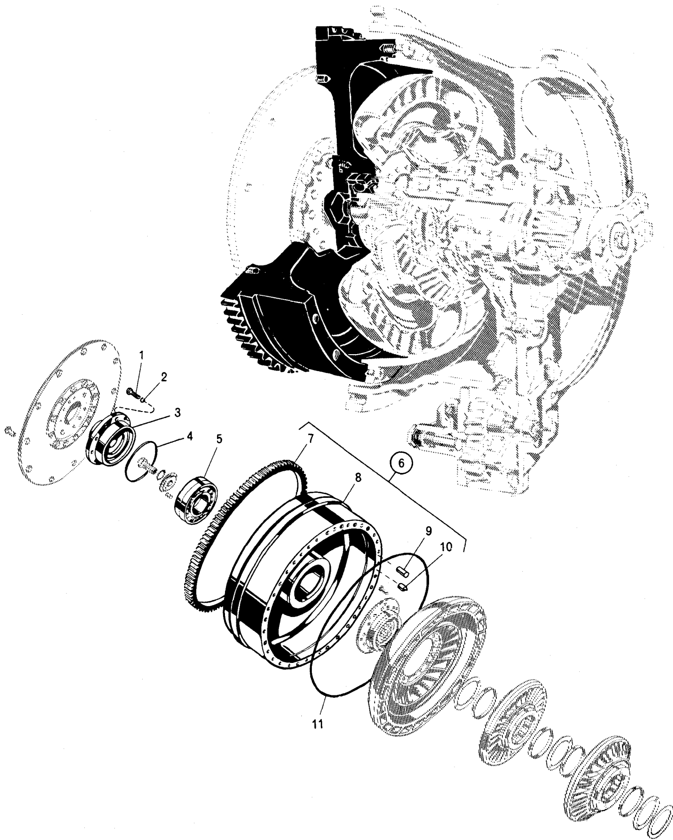
FIG. 6. FLYWHEEL
