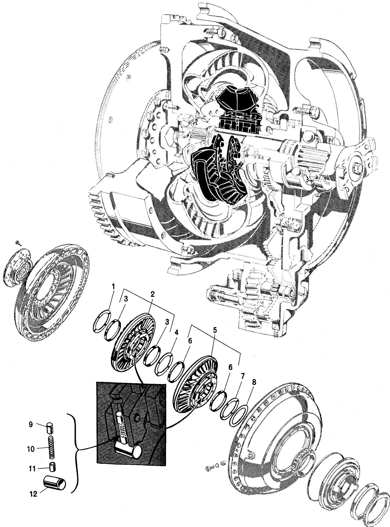
FIG. 3. STATOR
