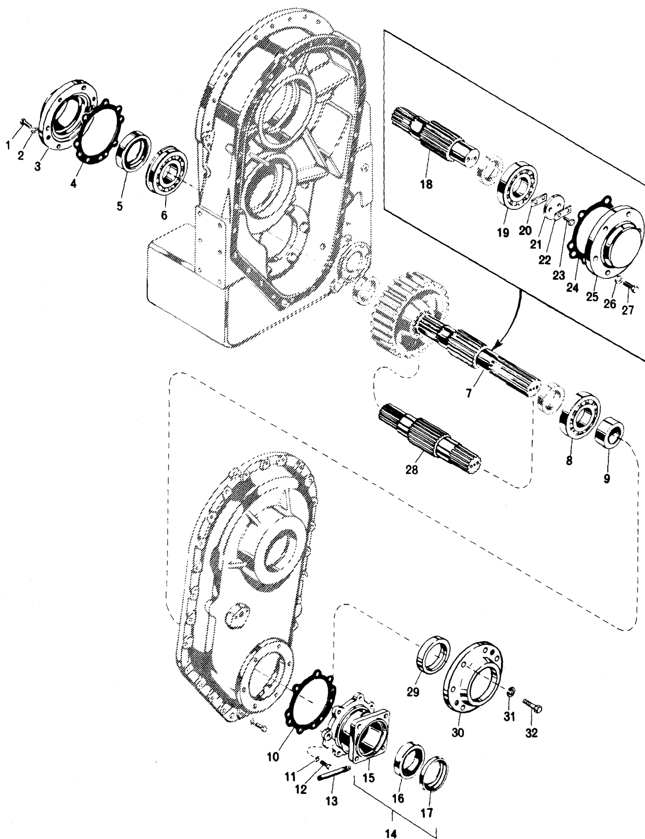
FIG 18 OUTPUT DRIVE
