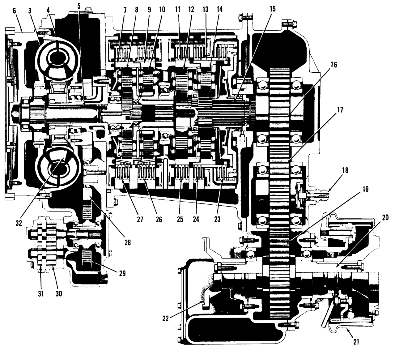
Model CRT 5631 Powershift Transmission Cross Section — Engine Mounted
