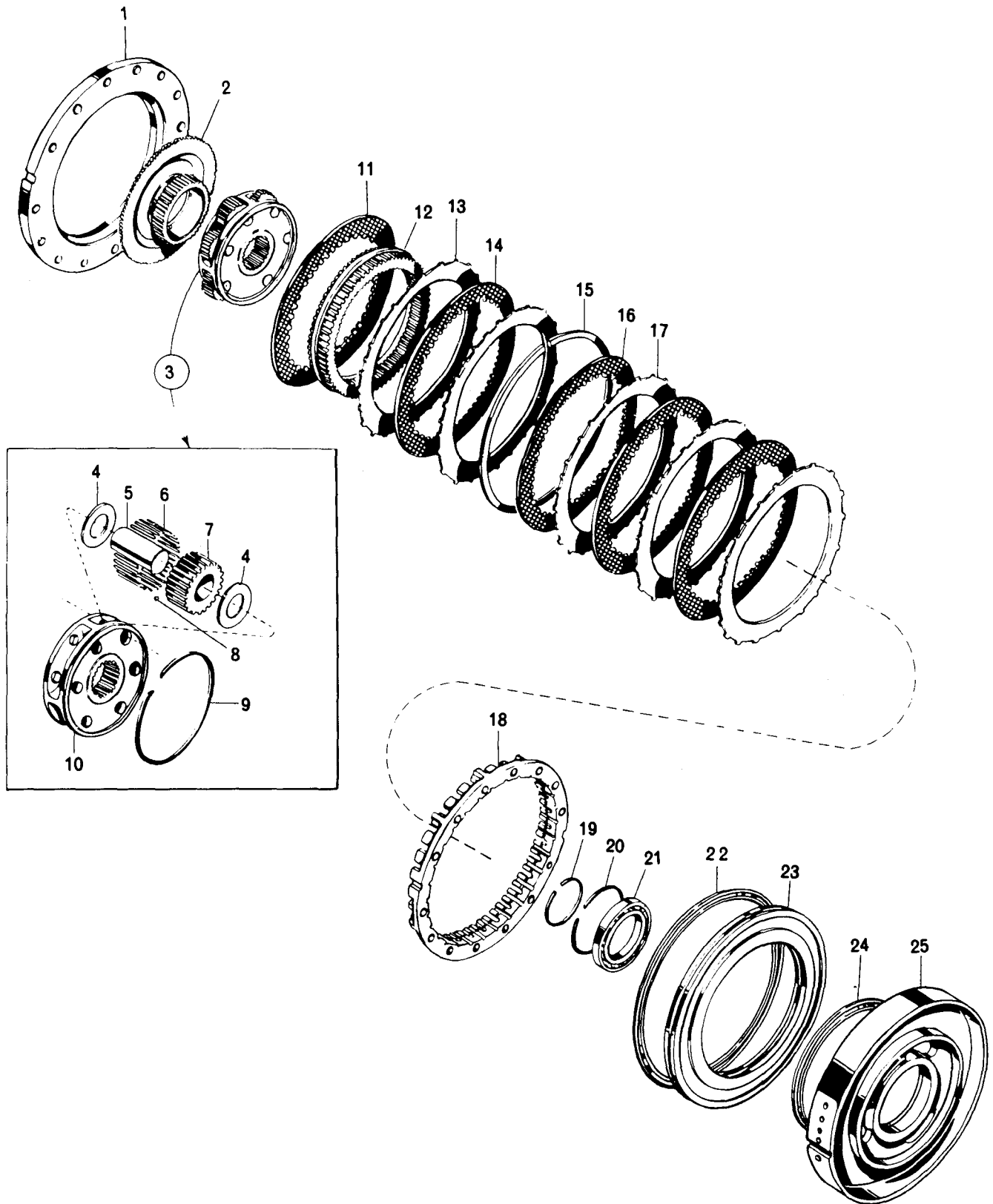
FIG 7-1 REVERSE PLANETARY AND CLUTCH
