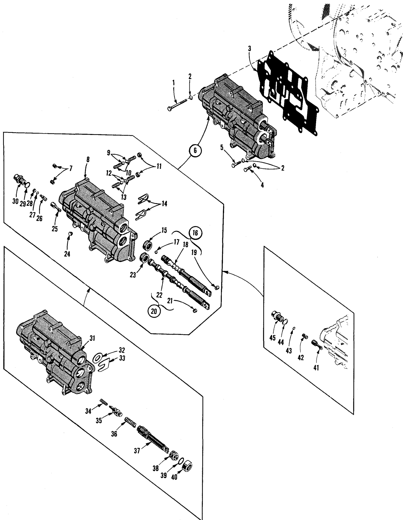
FIG XIX. CONTROL VALVE BODY, EXPLODED VIEW
