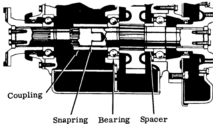
Fig. 2. Standard configuration
