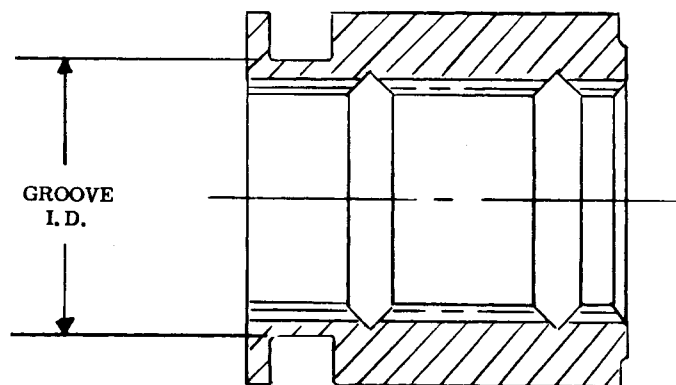
Figure 1. Disconnect Coupling
