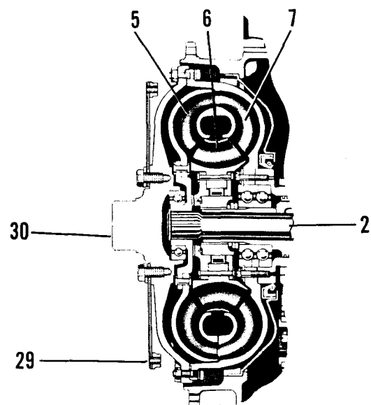
TRANSMISSION ENGINE MOUNTED (FLEX DISK DRIVE)
