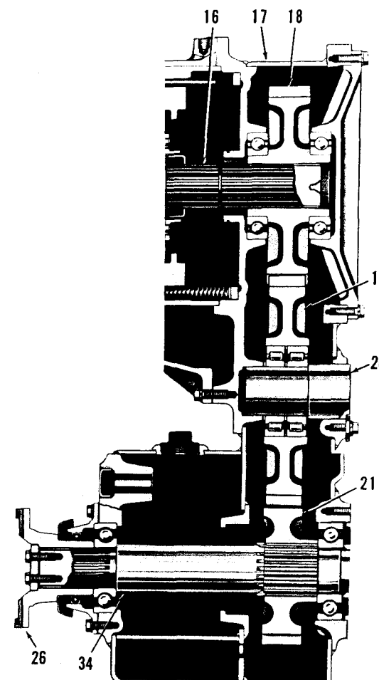
CRT3321-1 TRANSMISSION TRANSFER GEARS WITHOUT DISCONNECT
