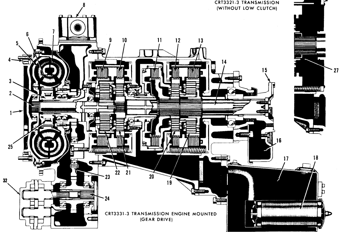
3321 and 3331-3 CROSS SECTION
