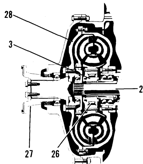
TRANSMISSION REMOTE MOUNTED (FLANGE DRIVE)
