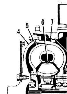
(ENGINE MOUNTED - FLEX DISK DRIVEN)
