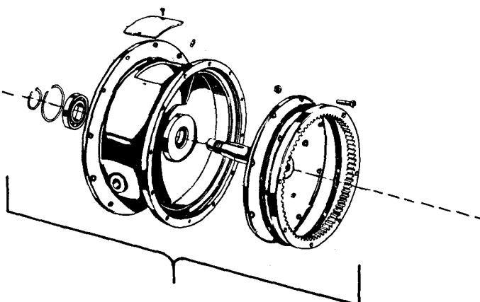
MANUAL INPUT DISCONNECT CLUTCH HOUSING OPTION
