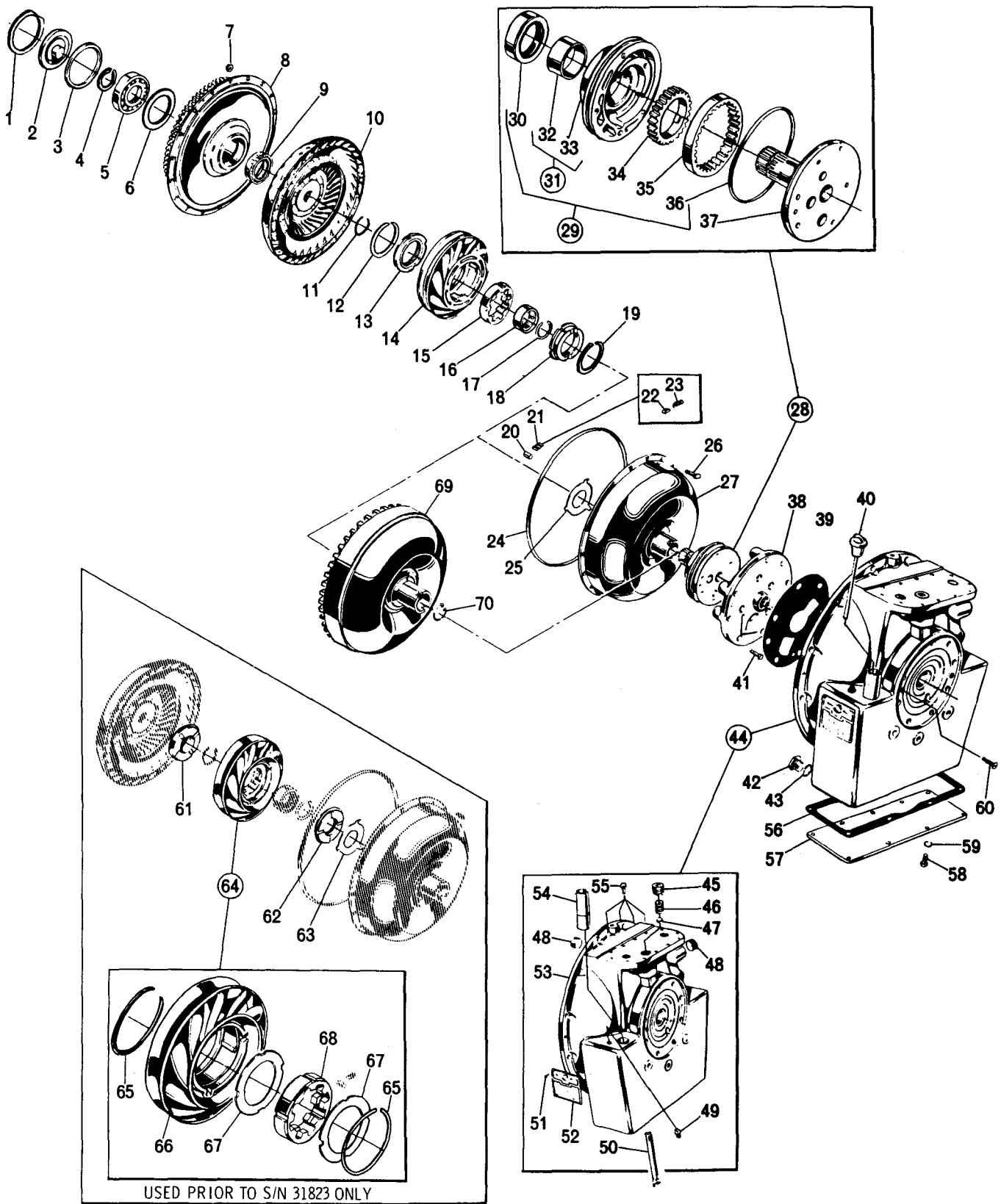
FIG. 1-1. TC 200 SERIES BASIC TORQMATIC CONVERTER WITH OVERRUNNING CLUTCH
