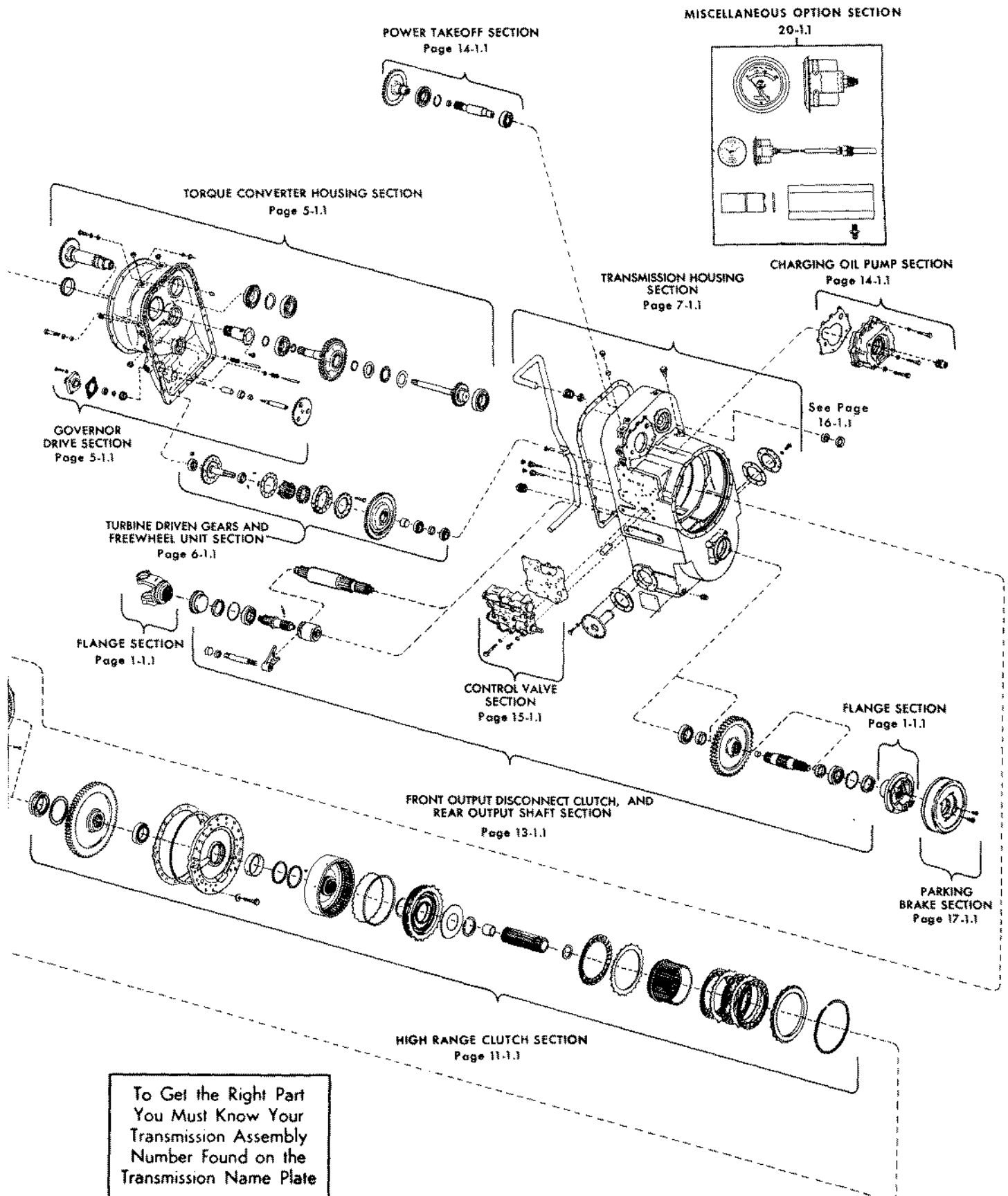
PICTORIAL INDEX (TRT-1 "LONG-DROP" TYPE)
