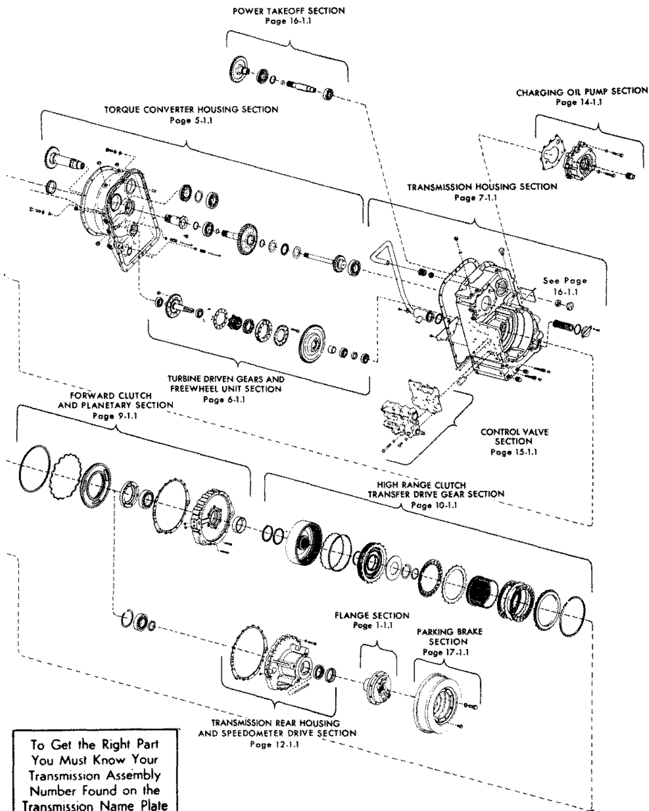
PICTORIAL INDEX (TRT-3 w/o OVERDRIVE "SHORT-DROP" TYPE)
