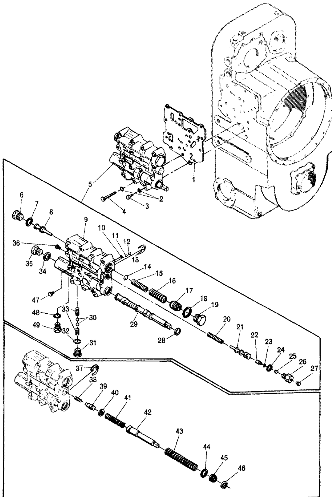
FIG. 15. CONTROL VALVE
