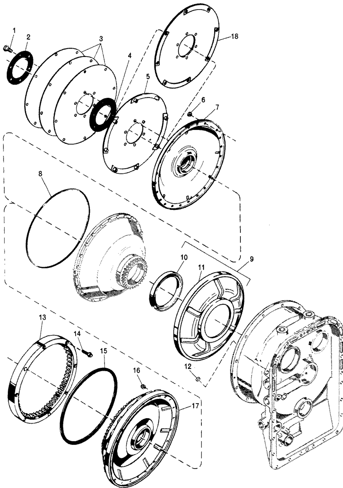
FIG. 3. FLEX DISK, CONVERTER DRIVE AND DRY CONVERTER TYPE HOUSING
