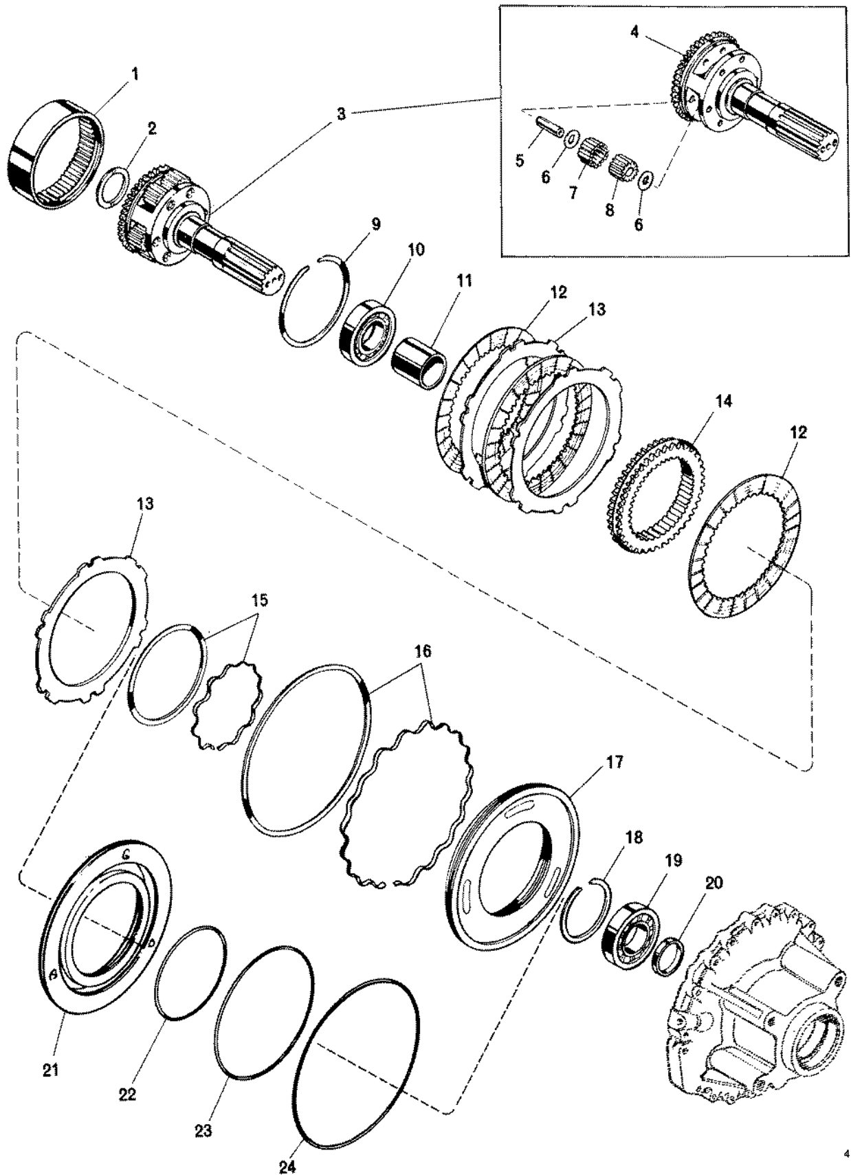
FIG. 9-2. FORWARD CLUTCH AND PLANETARY
