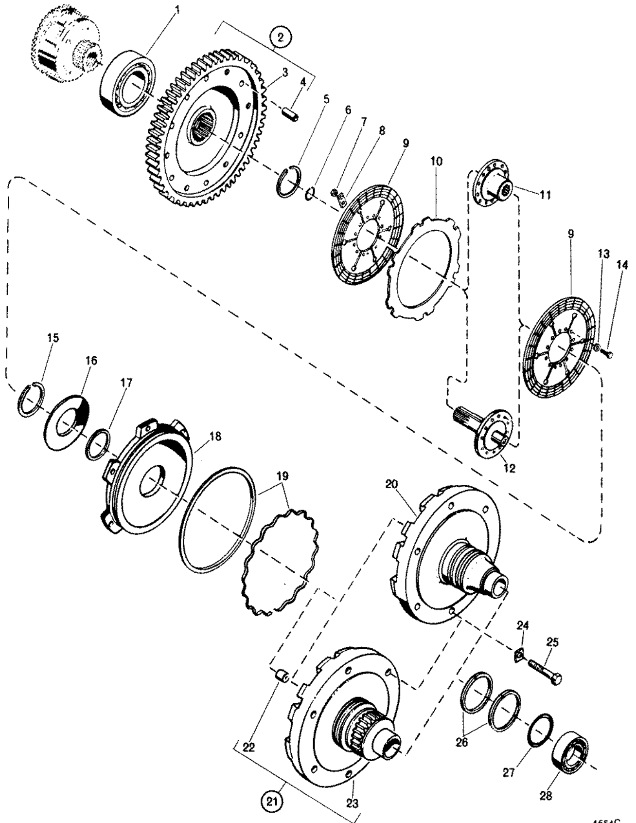
FIG. 10-4. HIGH-RANGE CLUTCH AND TRANSFER DRIVE GEAR
