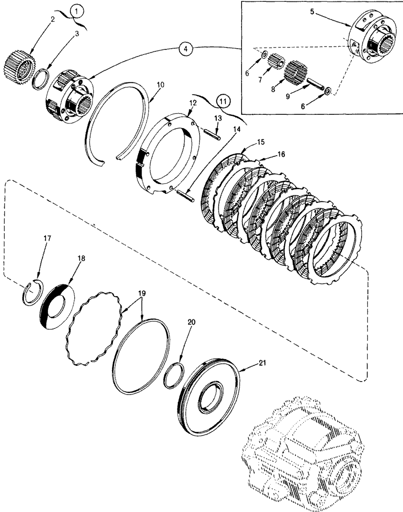
FIG. 10-3. HIGH-RANGE CLUTCH AND TRANSFER DRIVE GEAR
