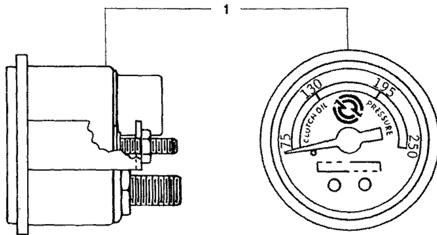
CLUTCH OIL PRESSURE GAGE
