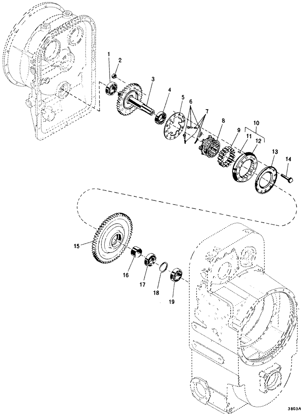
FIG. 6. TURBINE DRIVEN GEARS AND FREEWHEEL UNIT
