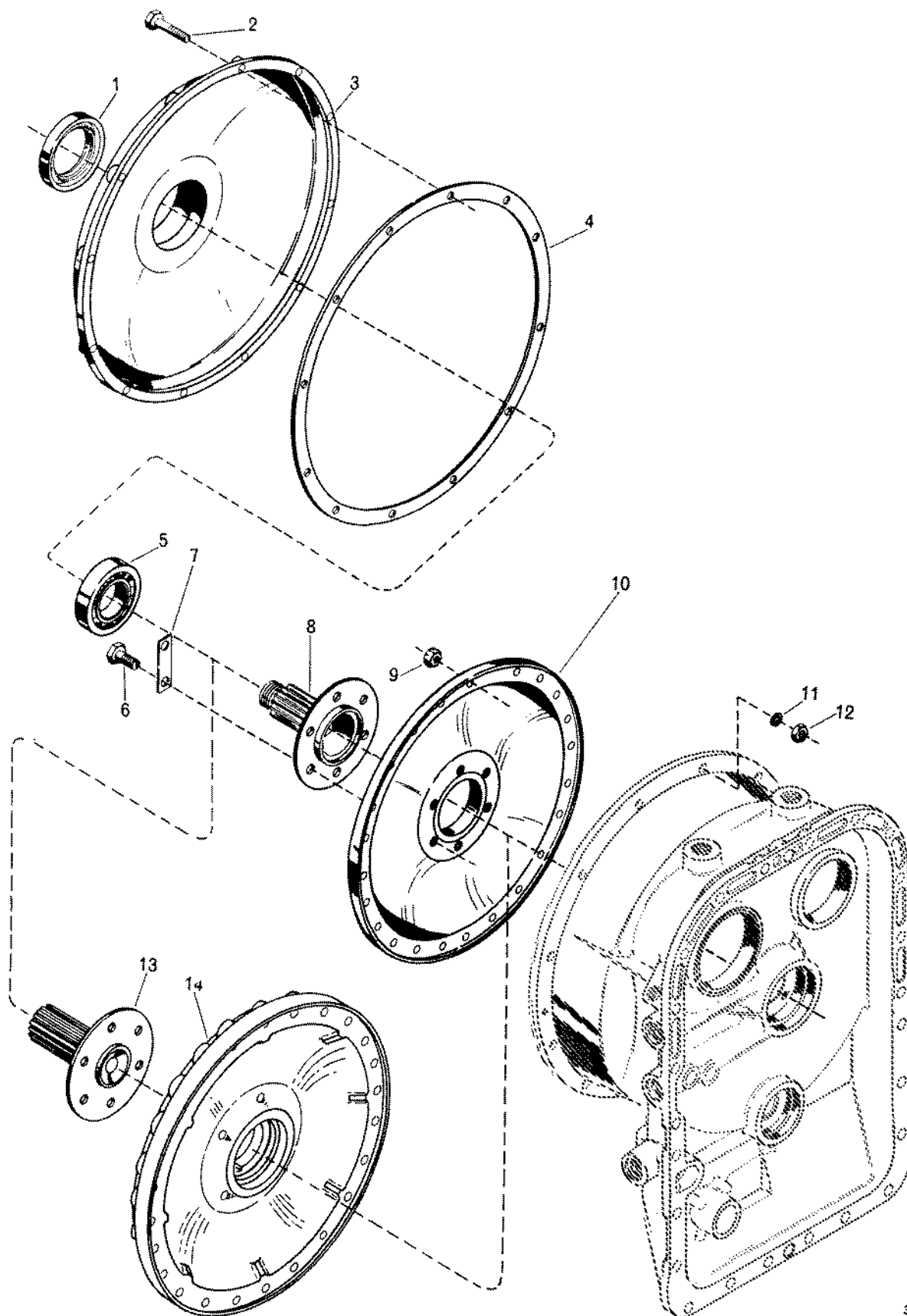
FIG. 2. TRANSMISSION FRONT COVER AND CONVERTER DRIVE
