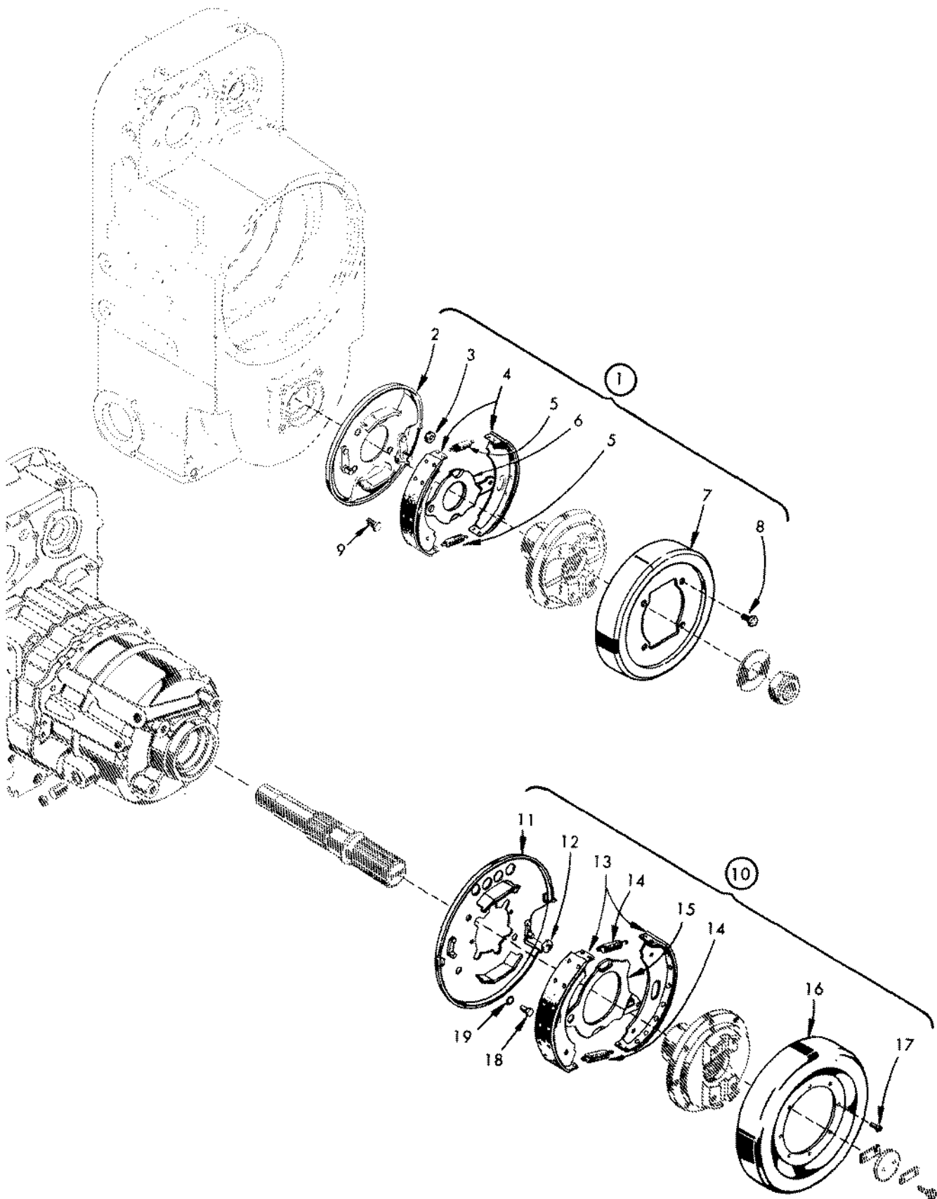
FIG. 17. PARKING BRAKE
