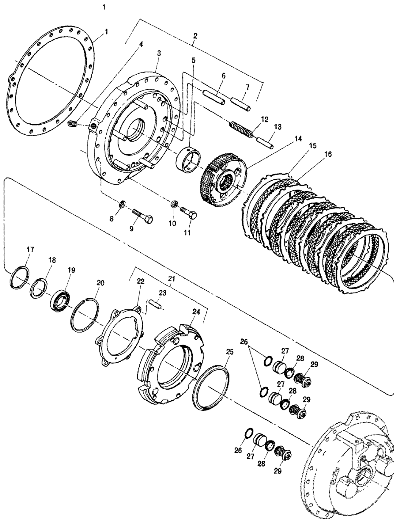
FIG. 19 INTERNAL SERVICE BRAKE
