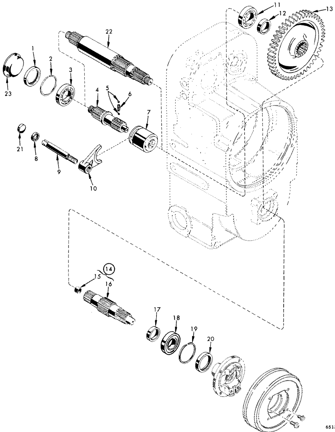
FIG. 13. FRONT OUTPUT DISCONNECT CLUTCH AND REAR OUTPUT SHAFT
