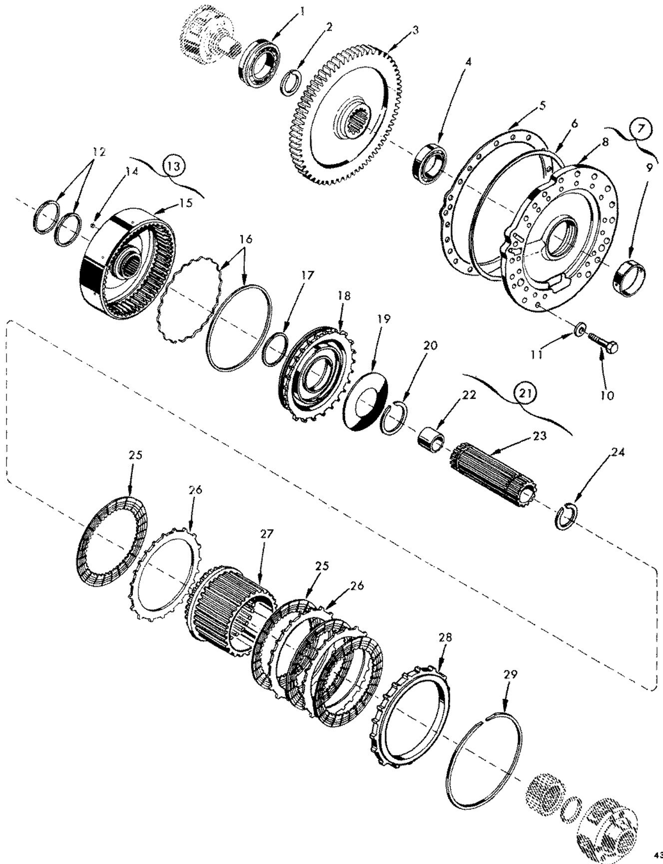
FIG. 11-2. LOW-RANGE CLUTCH AND PLANETARY
