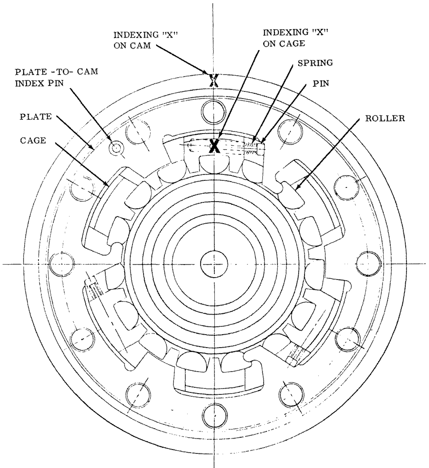
FIG. 2. CLUTCH SPRINGS AND PINS INSTALLED (SECTION A-A, FIG. 1)
