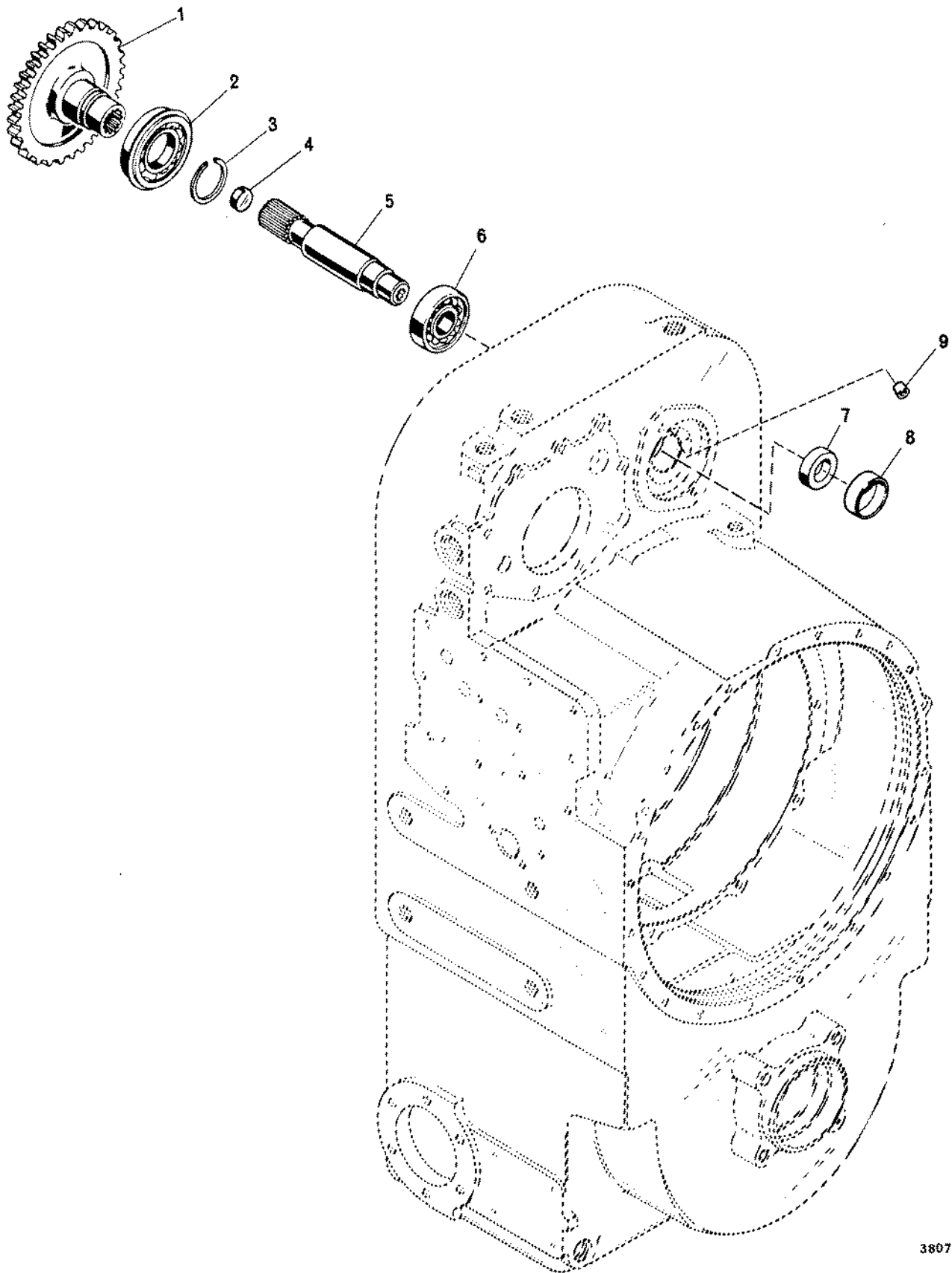
FIG. 16. POWER TAKEOFF
