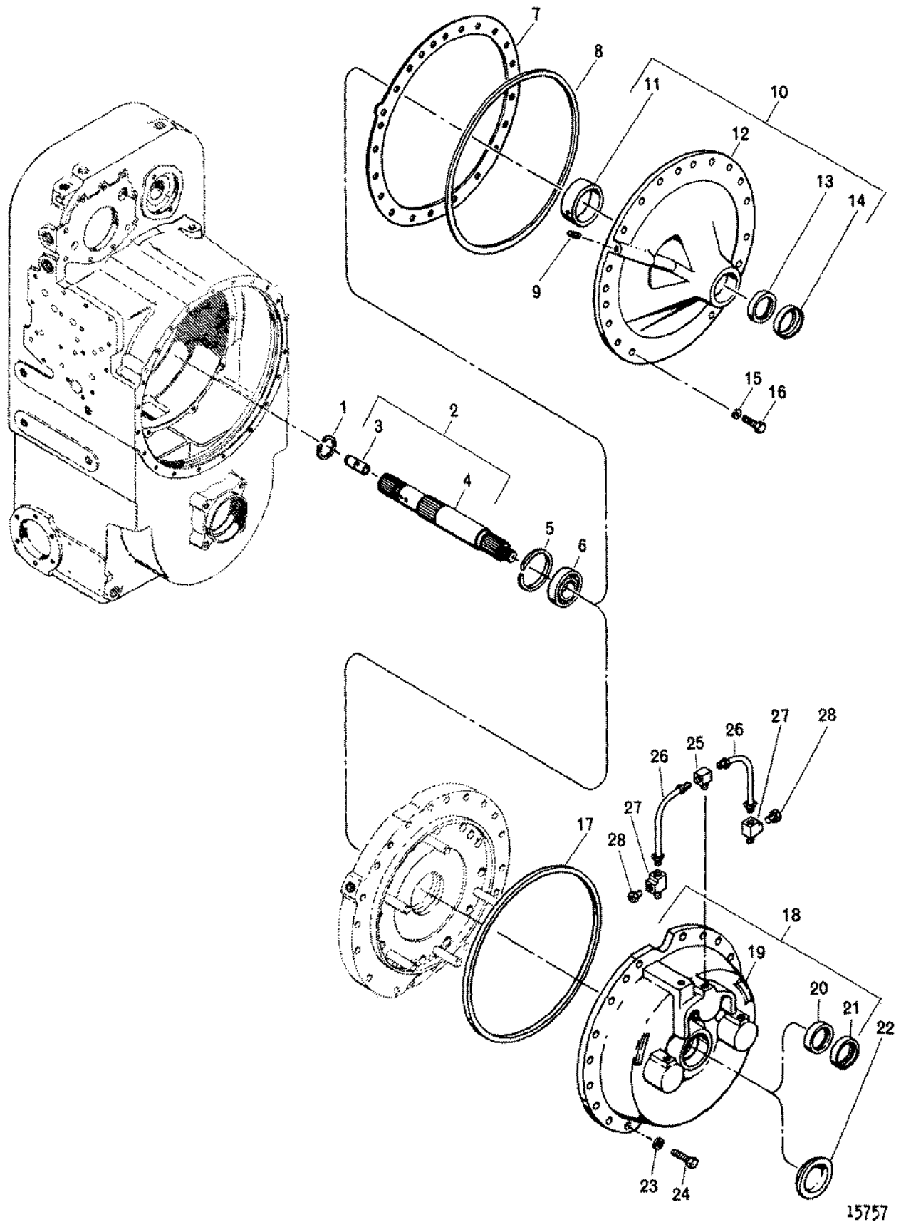
FIG. 12-2 TRANSMISSION REAR HOUSING AND SPEEDOMETER DRIVE
