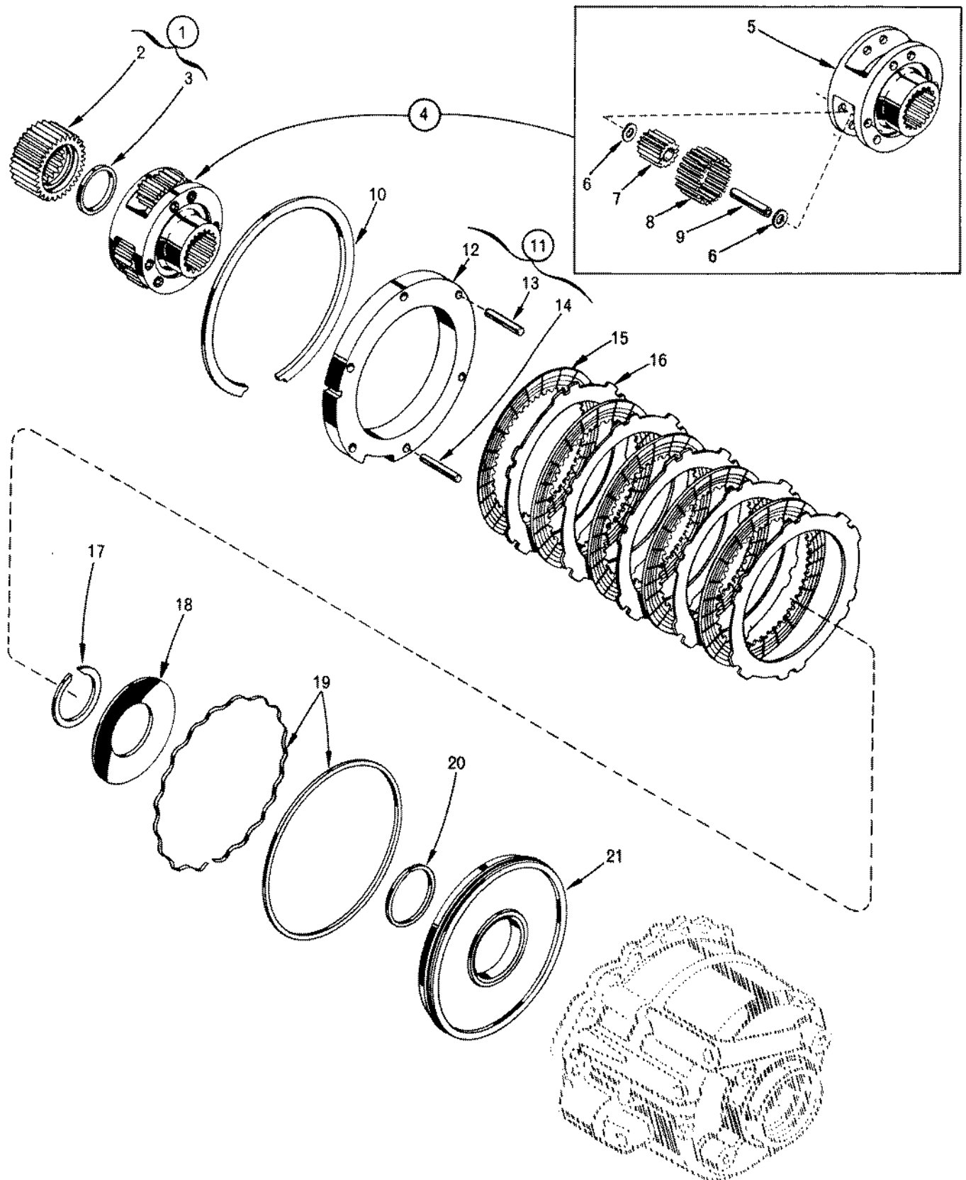
FIG. 11. LOW-RANGE CLUTCH AND PLANETARY
