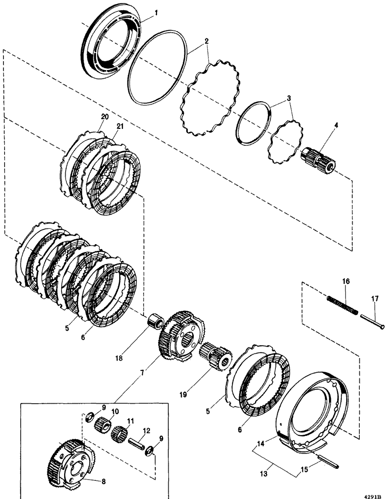
FIG. 8. REVERSE CLUTCH AND PLANETARY
