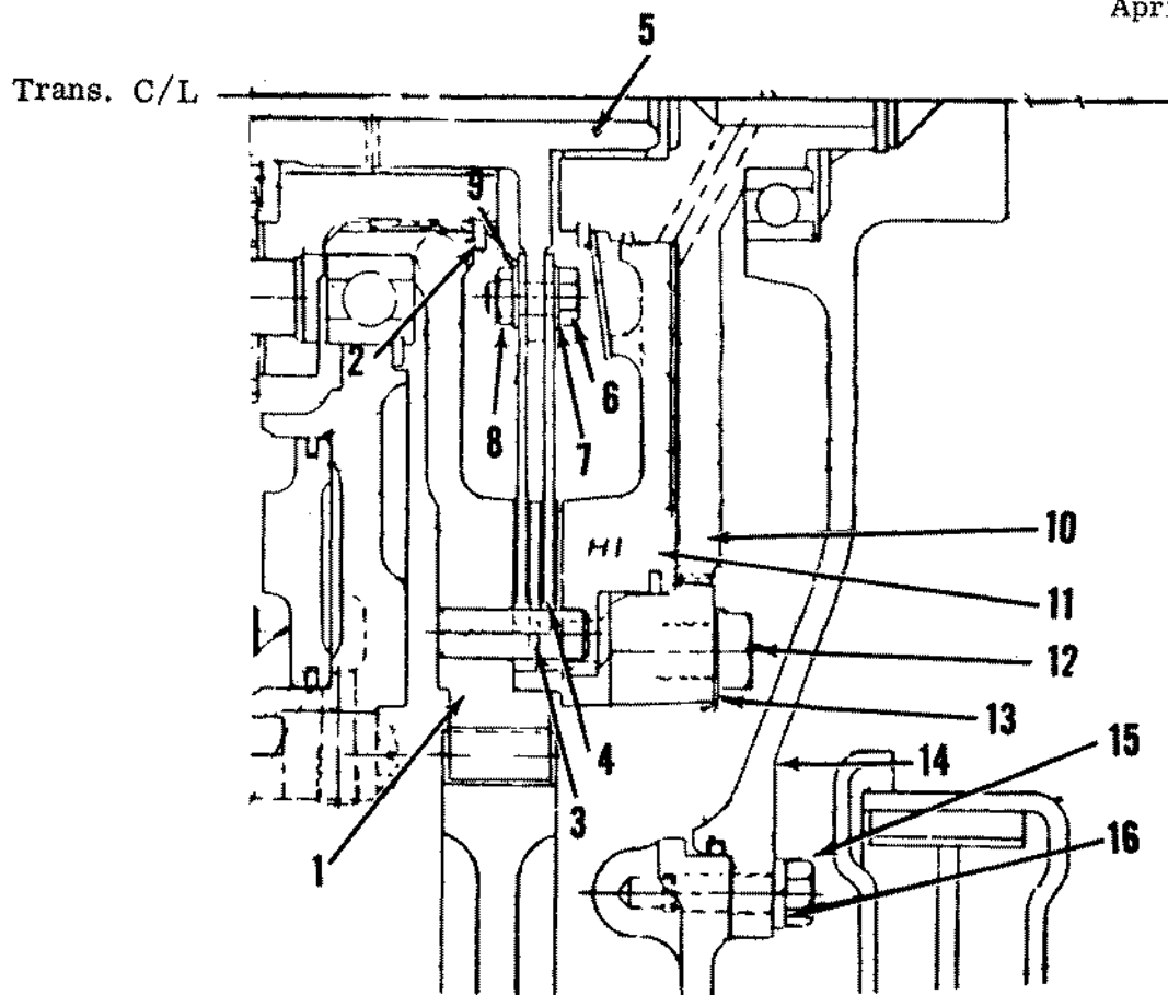
FIG. 1. HIGH CLUTCH - NEW CONFIGURATION
