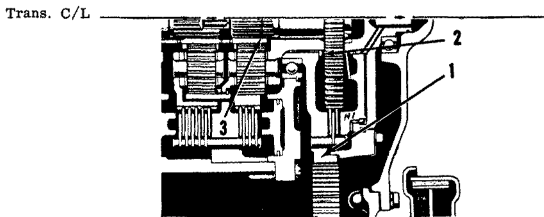
FIG. 1. HIGH CLUTCH - NEW CONFIGURATION
