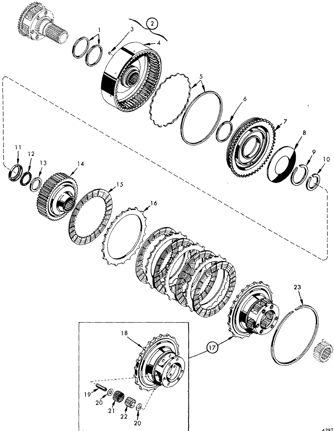
FIG. 11-1. LOW-RANGE CLUTCH AND PLANETARY
