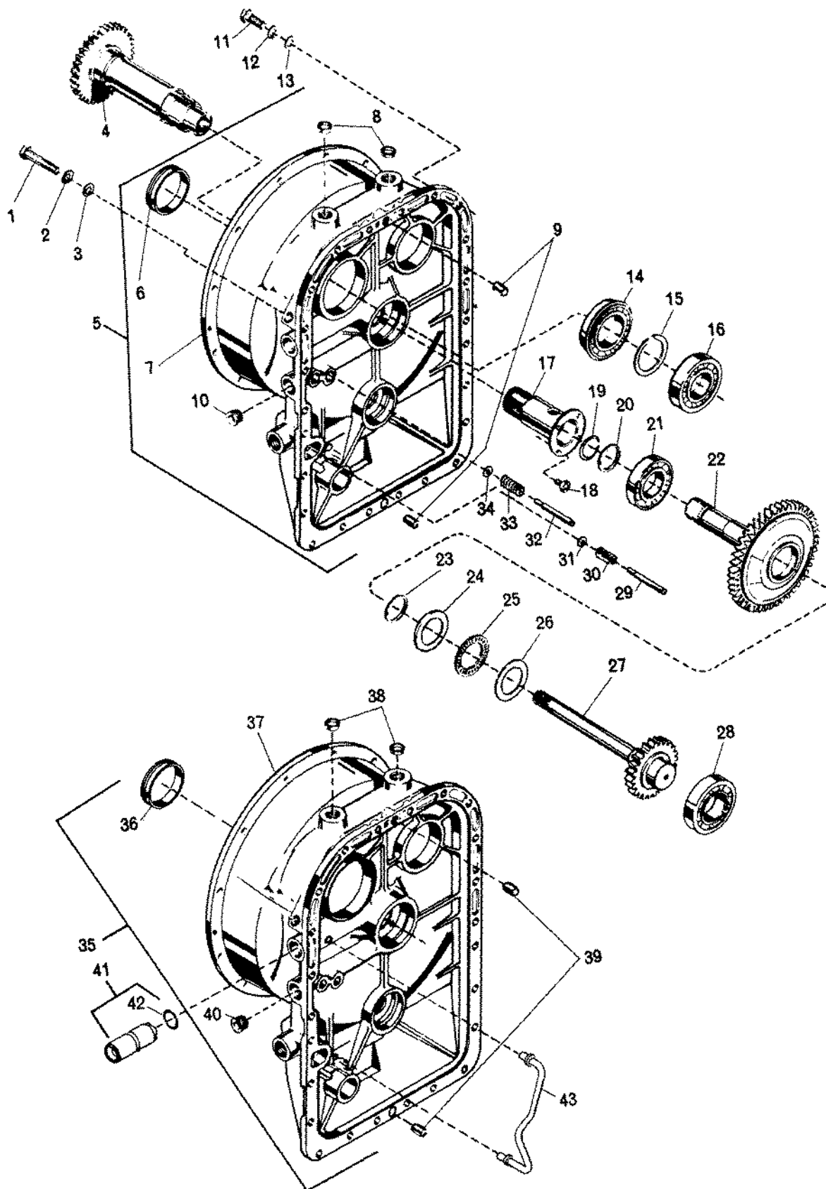
FIG. 5. TORQUE CONVERTER HOUSING
