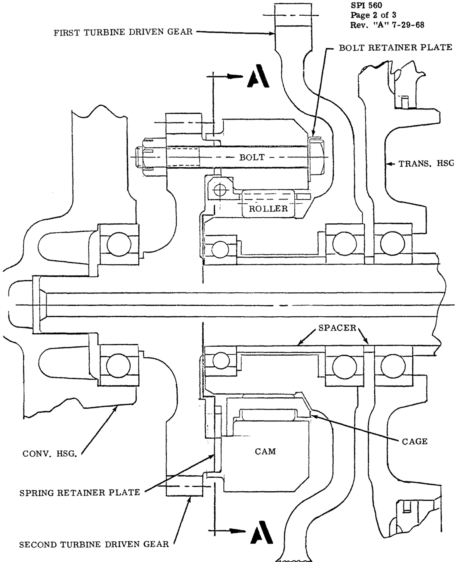
FIG. 1. FREEWHEEL CLUTCH ASSEMBLY - CROSS SECTION
