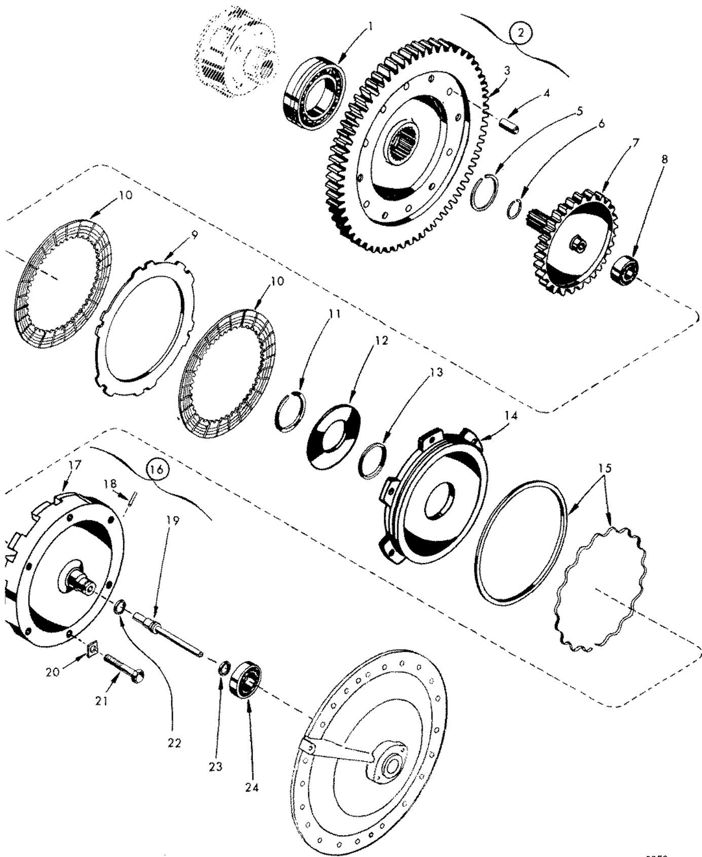
FIG. 10. HIGH-RANGE CLUTCH AND TRANSFER DRIVE GEAR
